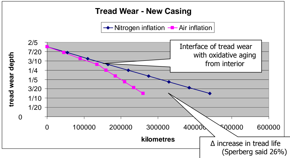
Figure 3: Expected tread wear – new casings
