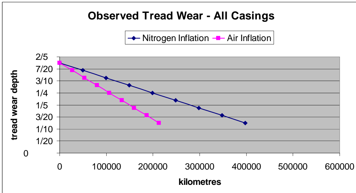
Figure 5: Actual tread wear – all trial casings
