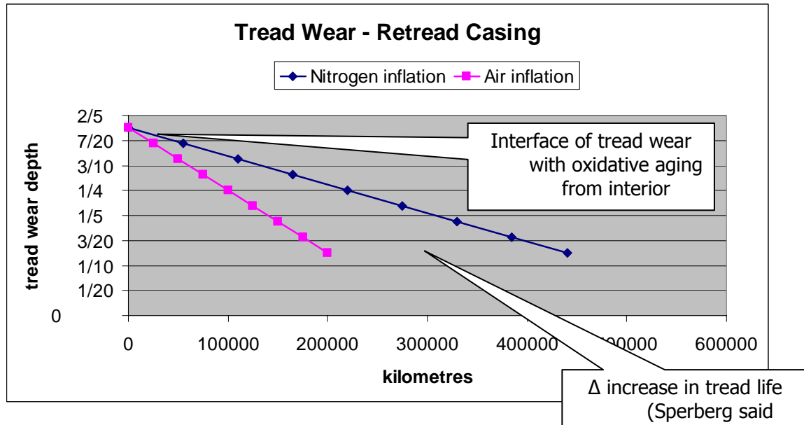
Figure 4: Expected tread wear – retreaded casings
