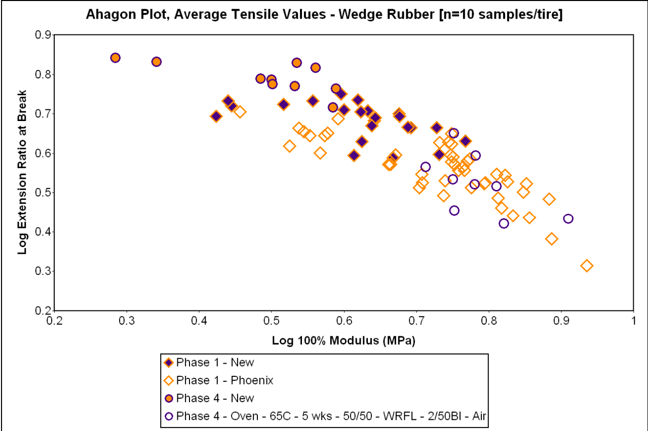
Figure 15: Changes in the Average Tensile Properties in the Wedge Rubber Region, New Tires, Phoenix Tires, & 5 Week Oven Aged Tires
