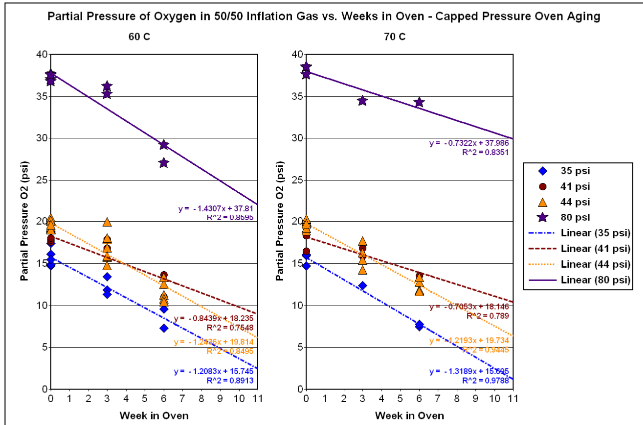
Figure 7: Partial Pressure of Oxygen in 50/50 Inflation Gas vs. Weeks in Oven for Capped Oven Aging at 60C & 70C
