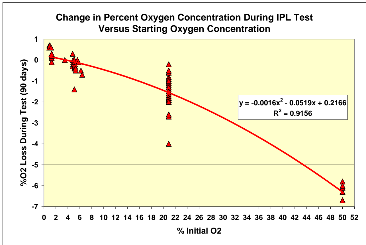
Figure 3: Percent O2 Change during Ninety Day Test versus Initial O2 Concentration
