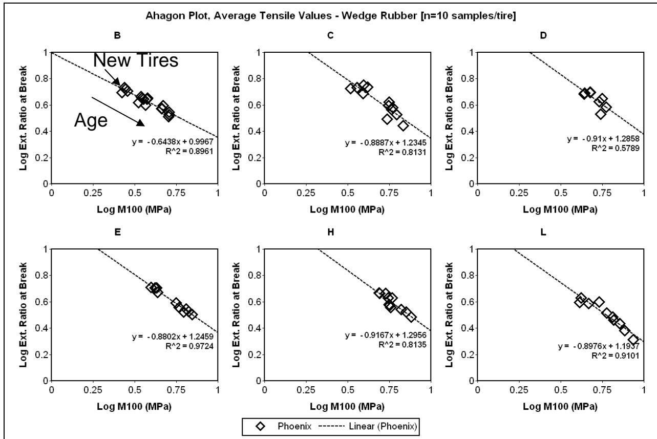
Figure 14: Changes in the Average Tensile Properties in the Wedge Rubber Region, New Tires & Phoenix Tires.
