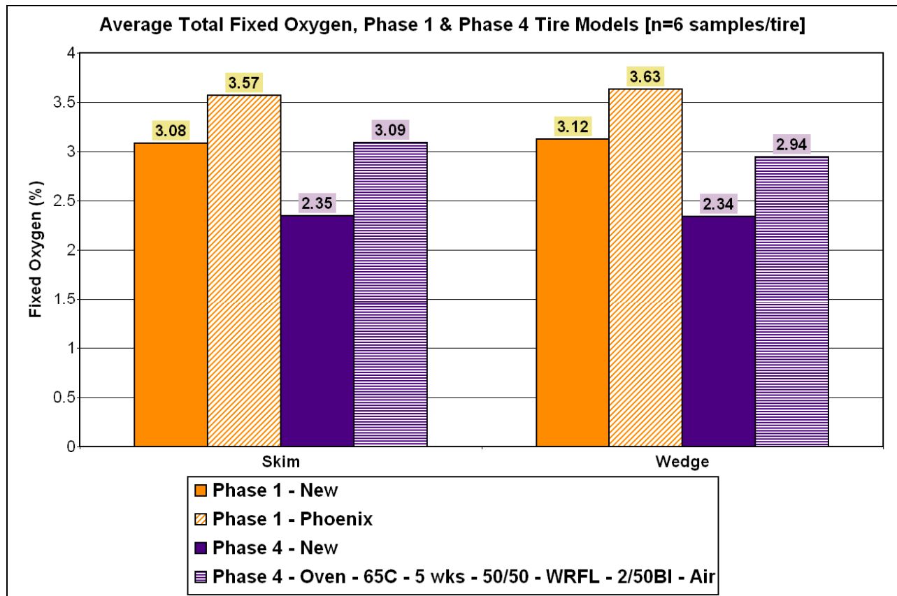
Figure 13: Changes in the Level of Fixed Oxygen in the Skim & Wedge Rubber Regions, New Tires, 5 Week Oven Aged Tires, Phoenix Tires
