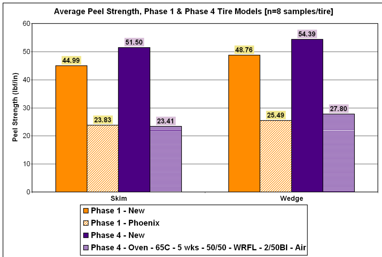
Figure 16: Changes in the Inter-Belt Peel Strength in the Skim & Wedge Rubber Regions, New Tires, Phoenix Tires, & 5 Week Oven Aged Tires
