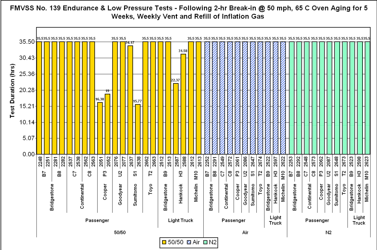
Figure 6: Tires Broken-in and Oven Aged with Various Inflation Gases vs. Performance in FMVSS No. 139 Endurance and Low Pressure Test Sequence
